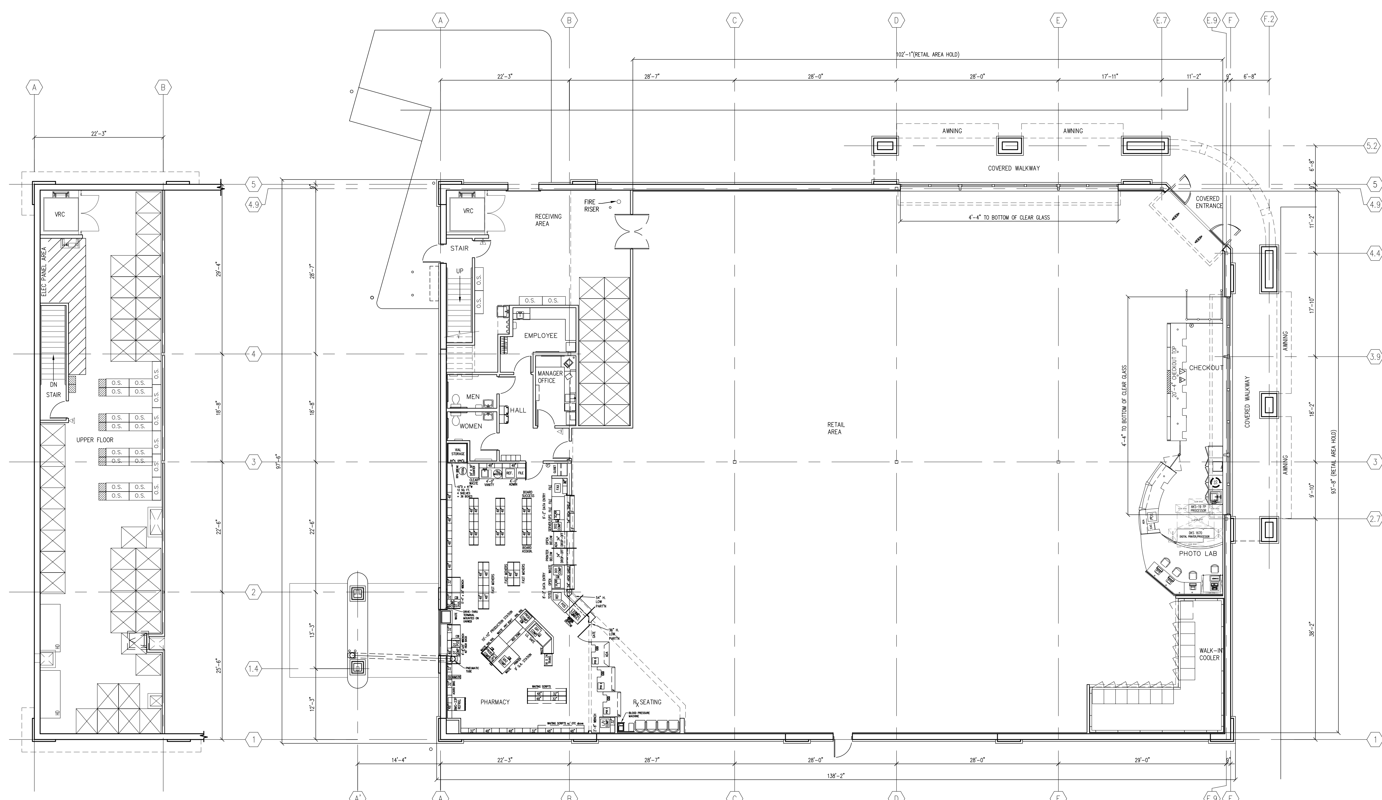
2 UPPER FLOOR PLAN 0-1 1/8" = 1'-0"
