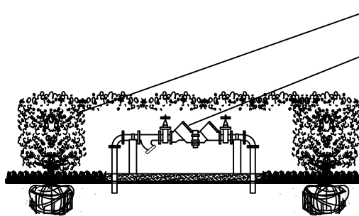
SECTION VIEW
