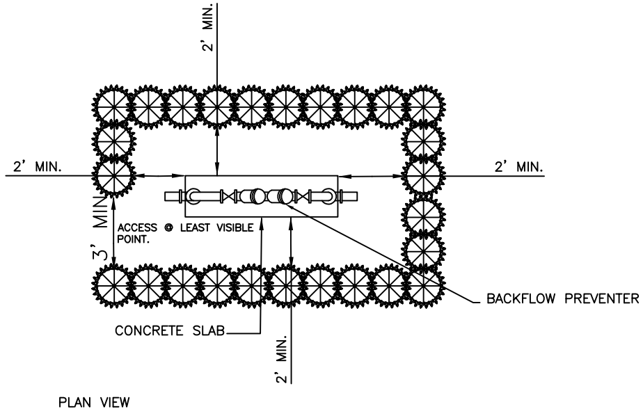
PLAN VIEW
